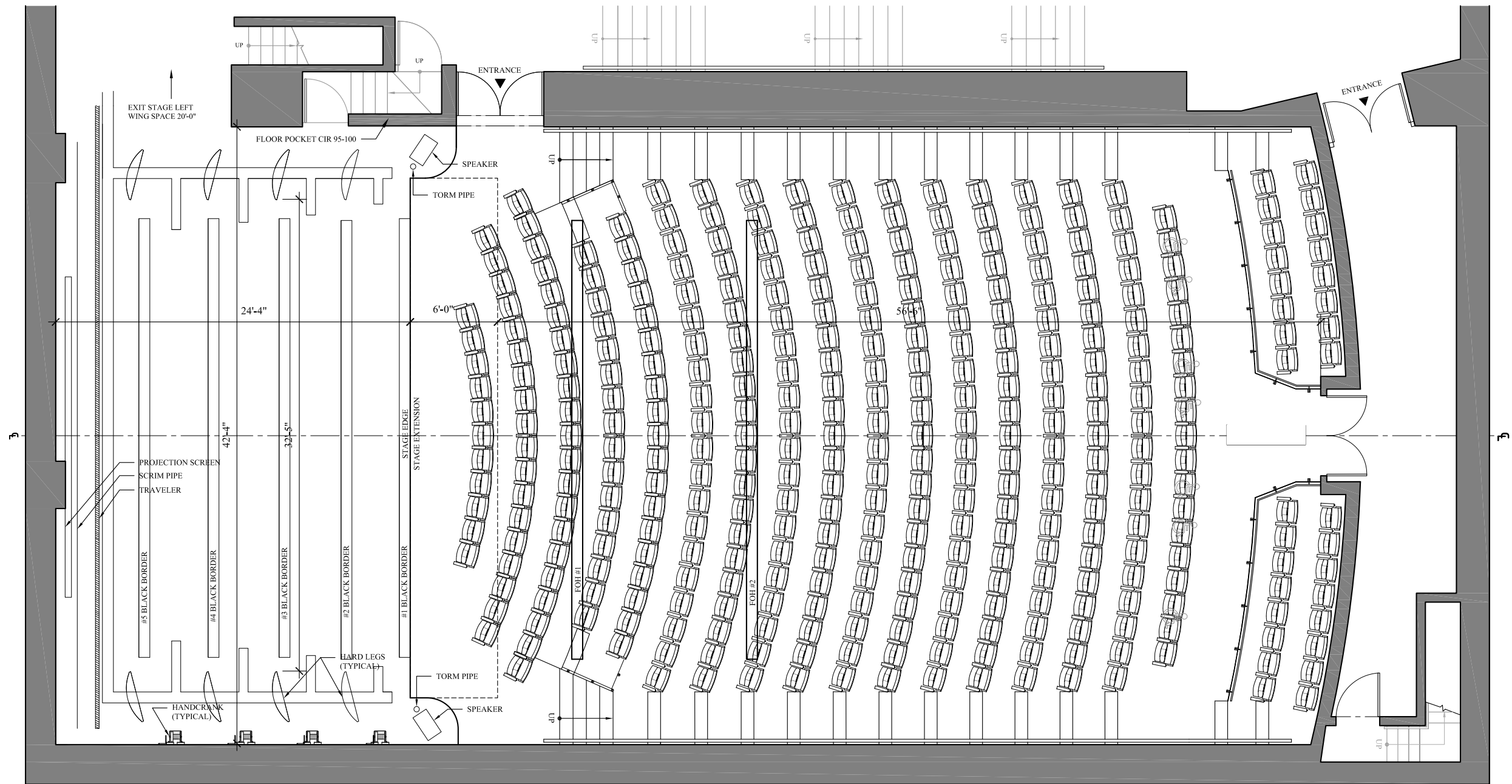
FRENCH INSTITUTE ALLIANCE FRANCAISE FLORENCE GOULD HALL PLAN VIEW WITH DIMENSIONS
